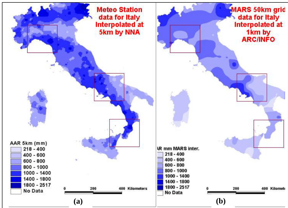
Figure 8. Average annual rainfall from (a) national meteorological network (366 stations) compared to (b) MARS 50km data interpolated to 1km, for Italy.
