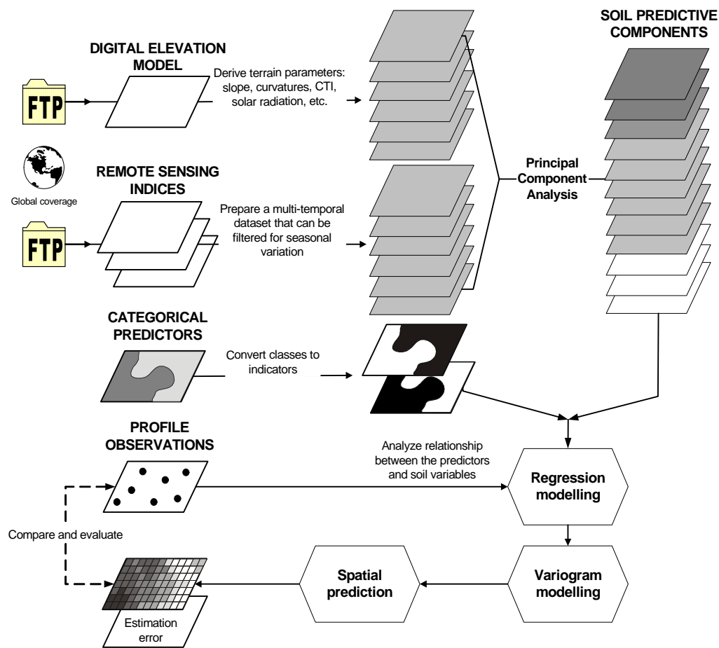
Fig. 2.2. Example of data-flow used to interpolate soil variables from profile observations using auxiliary information (the regression-kriging model).
