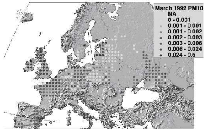
Fig. 3.6. PM10 emission in kg/m 2 for bare soil in the grid cell (example March 1992).
