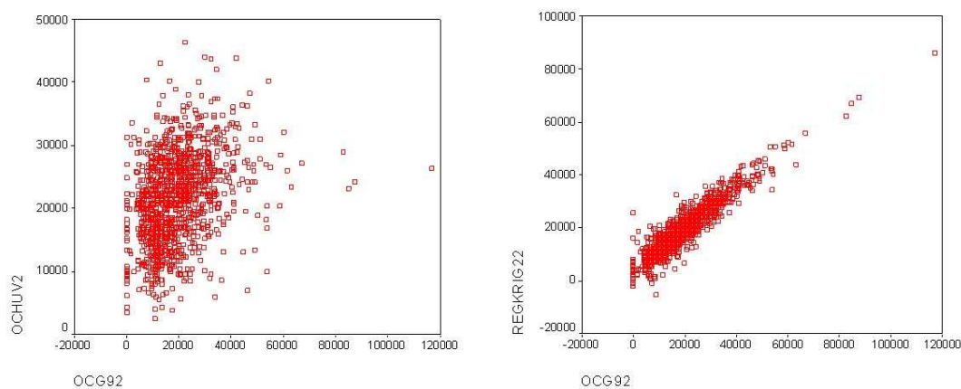
Fig. 3.9. Scatterplots of the original (OCG92) and the predicted SOM values for (a) the regression derived (OCHUV2) and (b) the regression-kriging derived (REGKRIG22) datasets.
