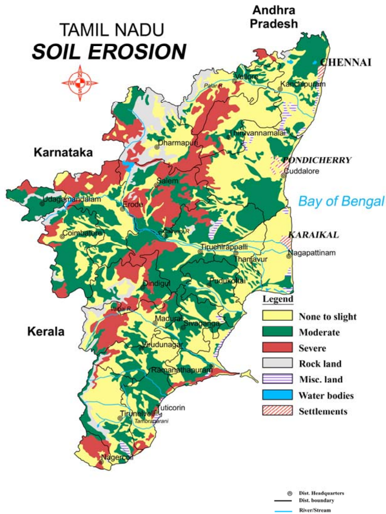
Fig. 2. Soil Map of erosion of Tamil Nadu region (NBSS & LUP, 1997)
