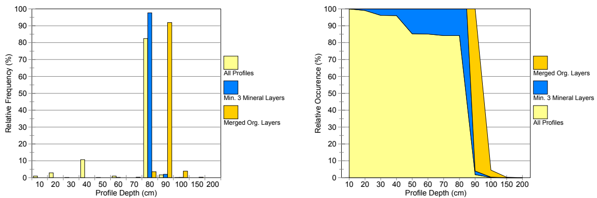
a) Profile Depth vs. Relative Frequency b) Profile Depth vs. Accumulated Relative Frequency
