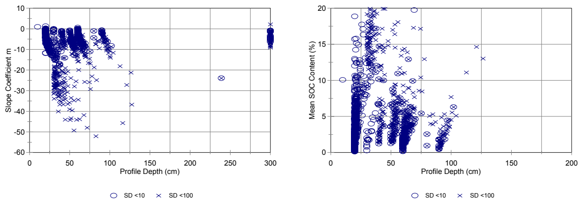
a) Profile Depth vs. Coefficient
