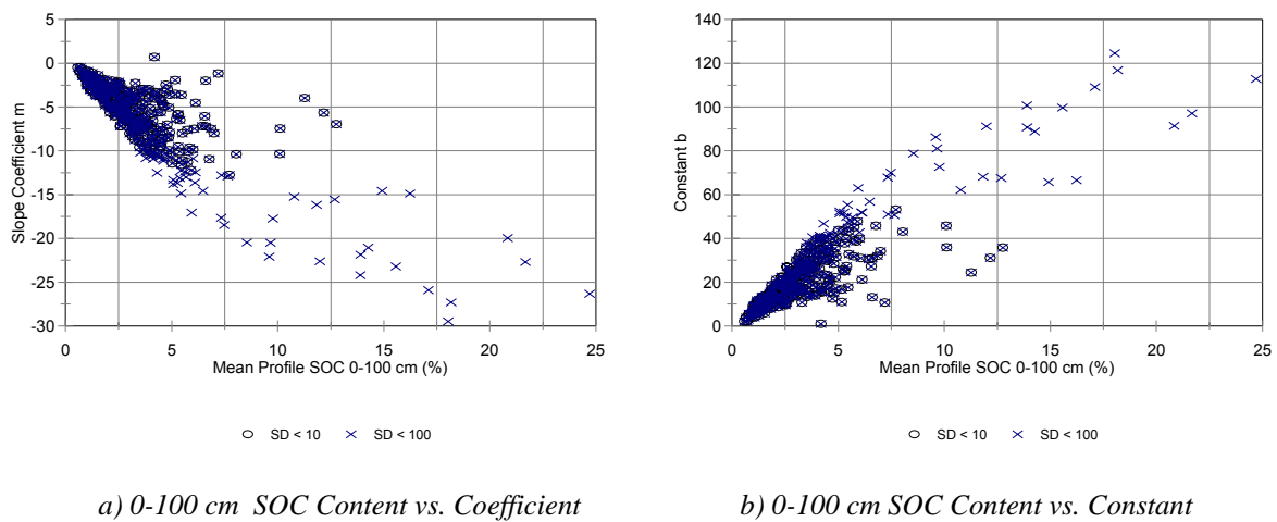
Figure 25: Relationship between Mean SOC Content and Model Slope Coefficient and Constant for Soil Section 0-100 cm Applying SD Threshold of 10 and 100 (Level II)
