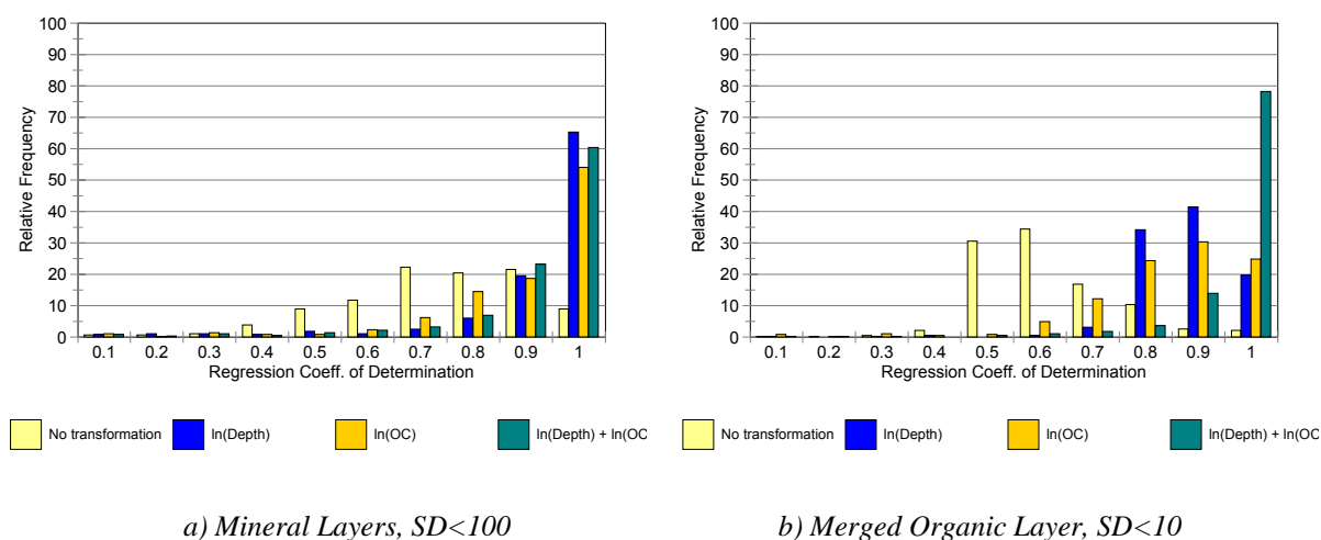
Figure 21: Frequency Distribution of Regression Coefficient of Determination for Logarithmic Transformation of SOC Content and Central Layer Depth for Mineral Layers and for Merged Organic Layers (Forest Focus Level II)
