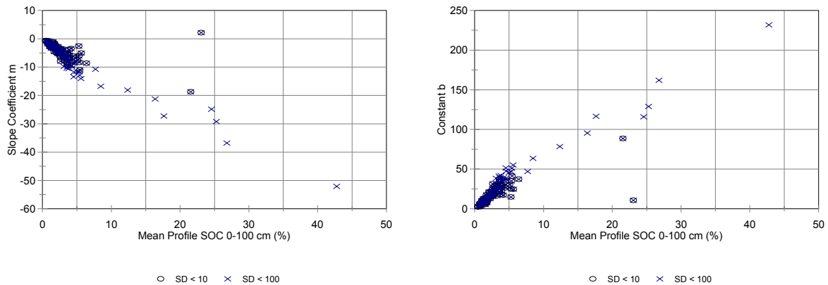
a) 0-100 cm SOC Content vs. Coefficient
