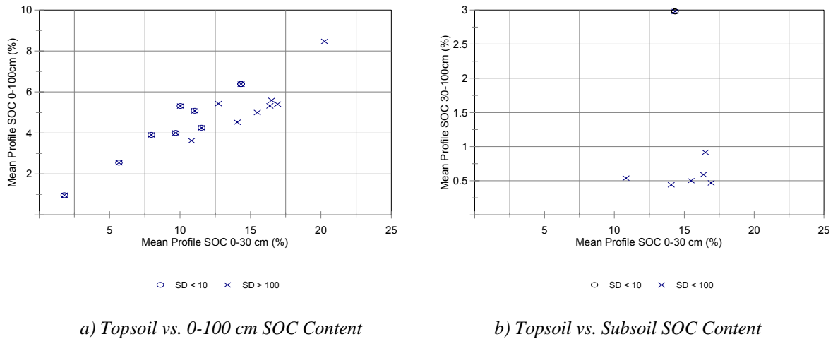
Figure 37: Relationship between Mean SOC Content in Topsoil and Soil Segment 0-100 cm and Subsoil (Level I)
