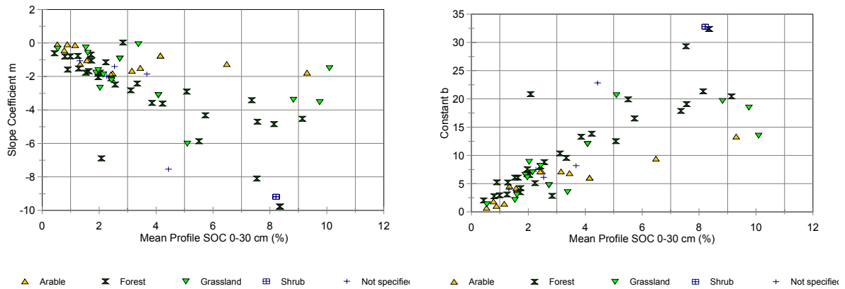
a) Topsoil SOC Content vs. Coefficient
