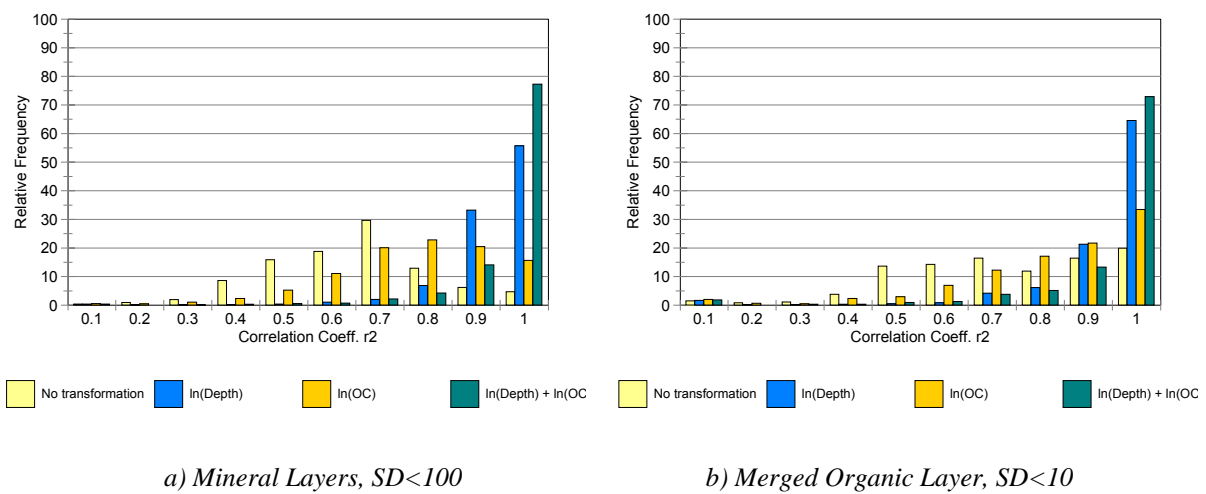
Figure 35: Frequency Distribution of Regression Coefficient for Logarithmic Transformation of SOC Content and Central Layer Depth for all Layers and for Merged Organic Layers (Forest Focus Level I)
