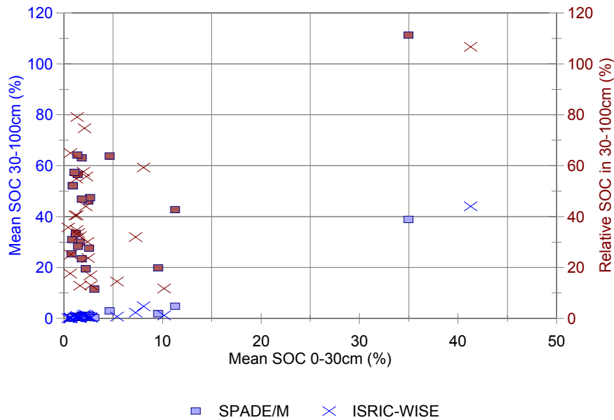
Figure 66: Relationship between Soil Organic Carbon Content in the 0-30 cm Topsoil Layer and the 30-100 cm Subsoil Layer for SPADE/M and ISRIC-WISE Major Soil Types
