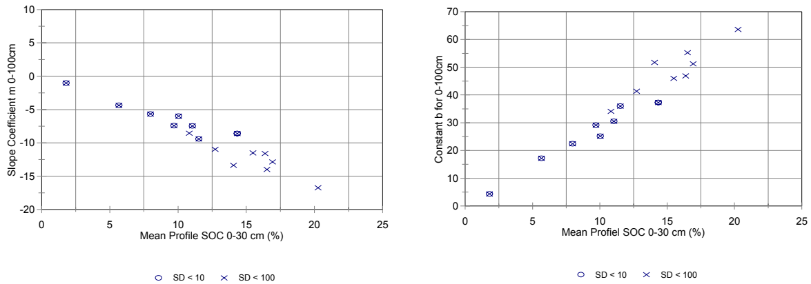
a) Topsoil SOC Content vs. 0-100 cm Coefficient b) Topsoil SOC Content vs. 0-100 cm Constant
