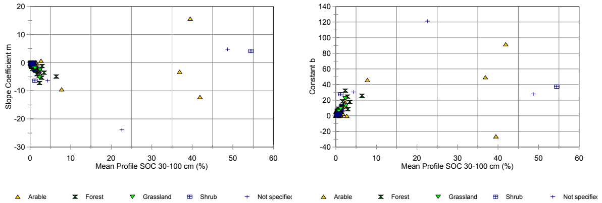
a) Subsoil SOCC Content vs. Coefficient
