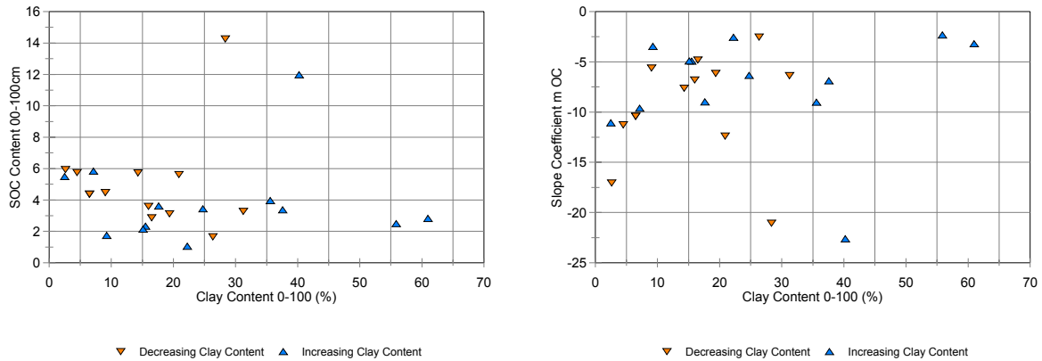
a) 0-100 Clay vs. 0-100 cm SOC Content
