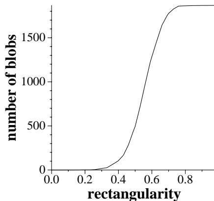
Fig. 5. Number of blobs vs rectangularity threshold
