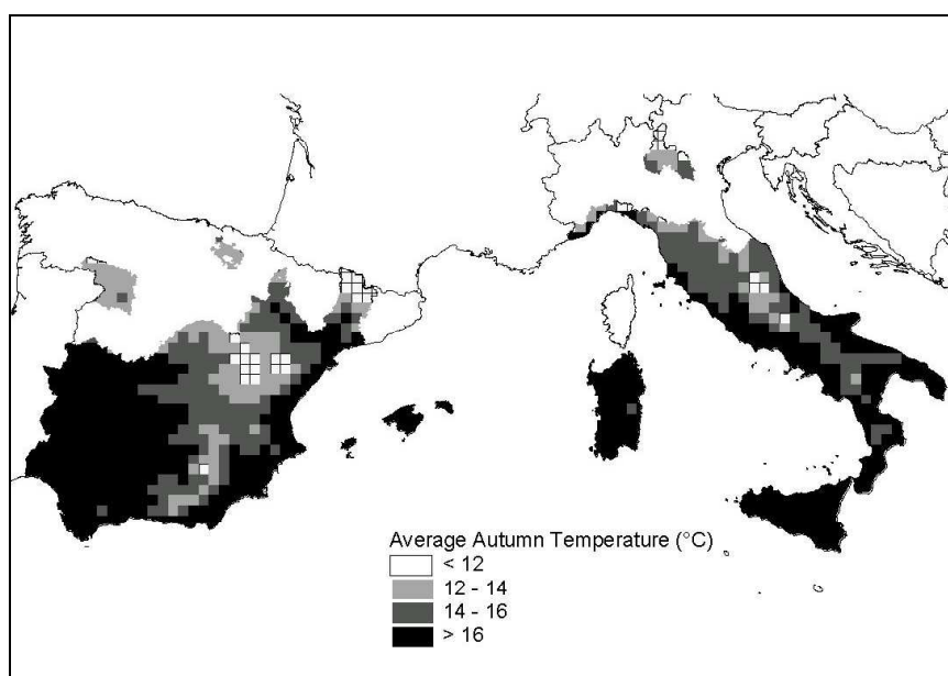
Figure A1.4. Average autumn temperature
