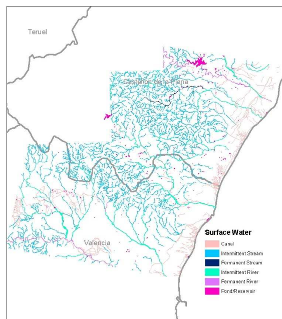
Figure A4.5. Surface water (1:25 000 scale) in the Valenciana region from MTN25 digital data
